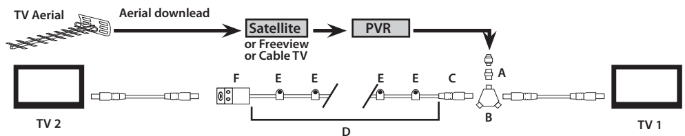
Fig. 2 - TV Aerial / Video / Satellite / Cable TV / Freeview
